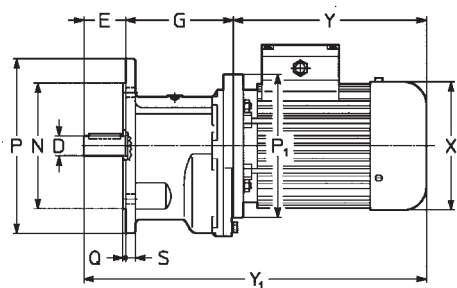
Standard design 1) Mounting position B5, V1, V3
